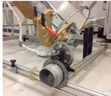
Motorized solar tracker with wire transmission
